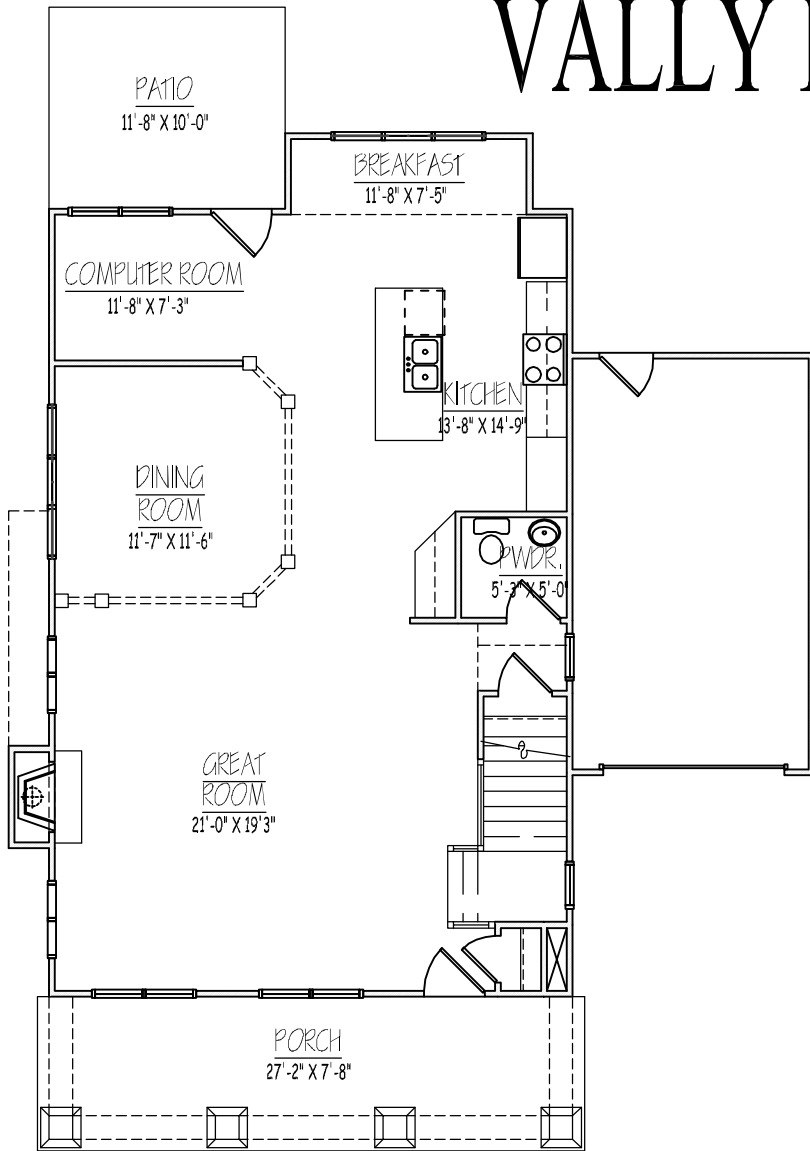
FIRST FLOOR GARAGE OPT.
